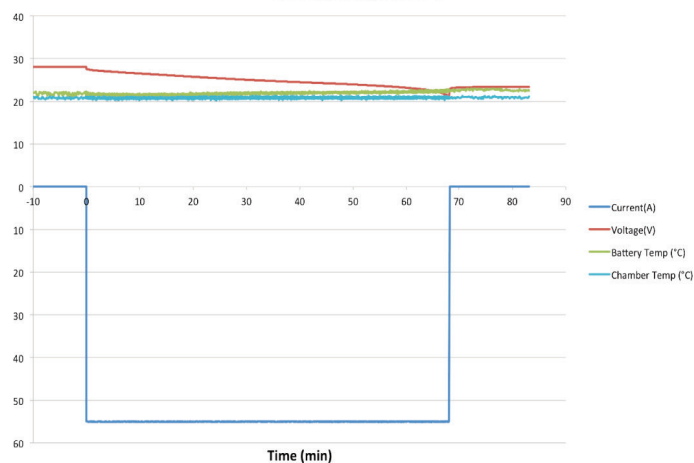
55A Discharge at 20°C
