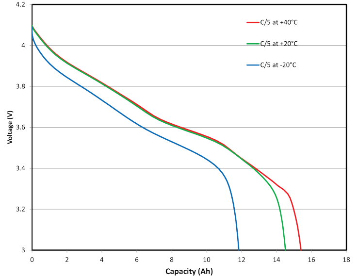
Discharge Rate at C/5 and Various Temperatures
