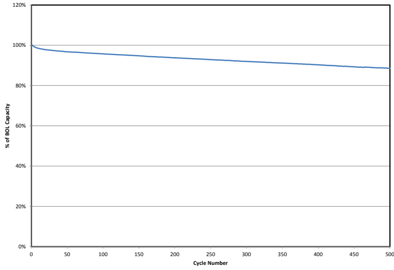
Contego 3 Cycle Life at 37°C and C/2
