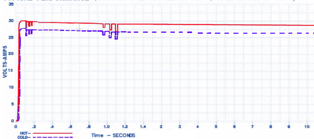
TYPICAL PERFORMANCE (RISE TIME COLD 0.040 SEC TO 16.0 V, HOT 0.020 SEC TO 16.0 V)
